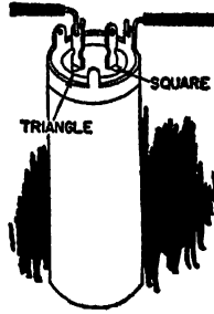
Electrolytic capacitor in metal can. Square and triangular cut-outs in insulating wafer identify the terminal lugs.
